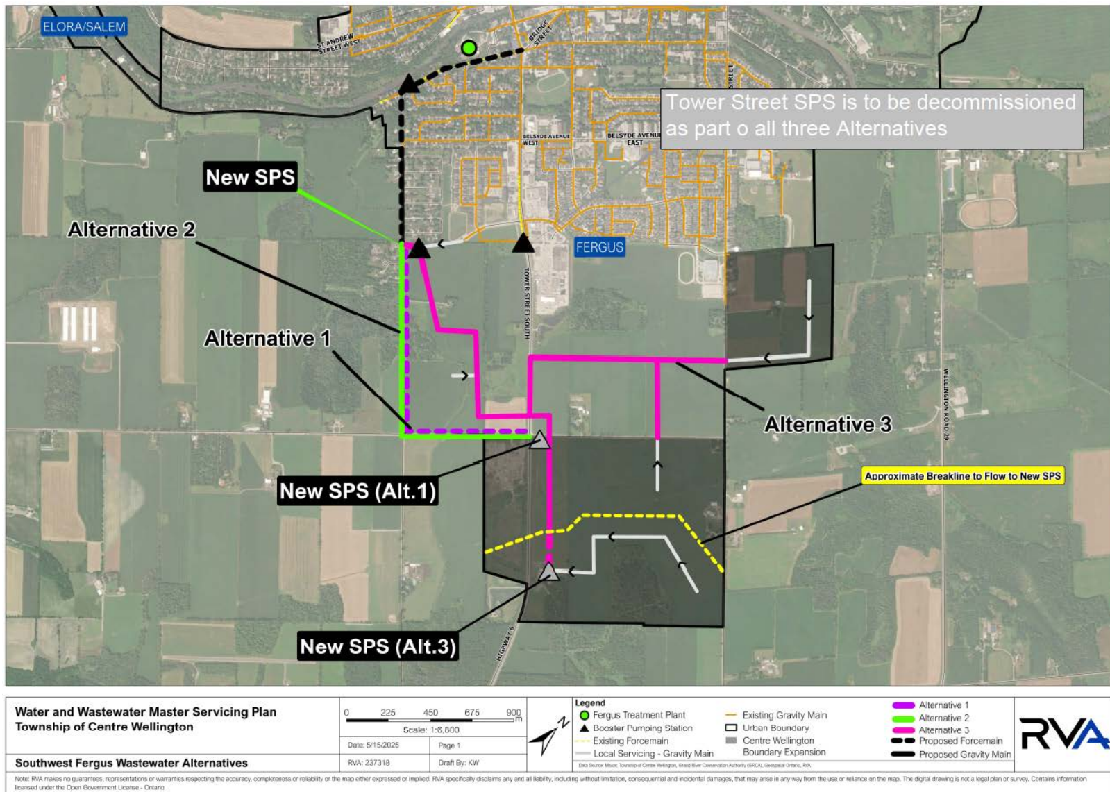
Figure 7-13 South Fergus Collection System Options
