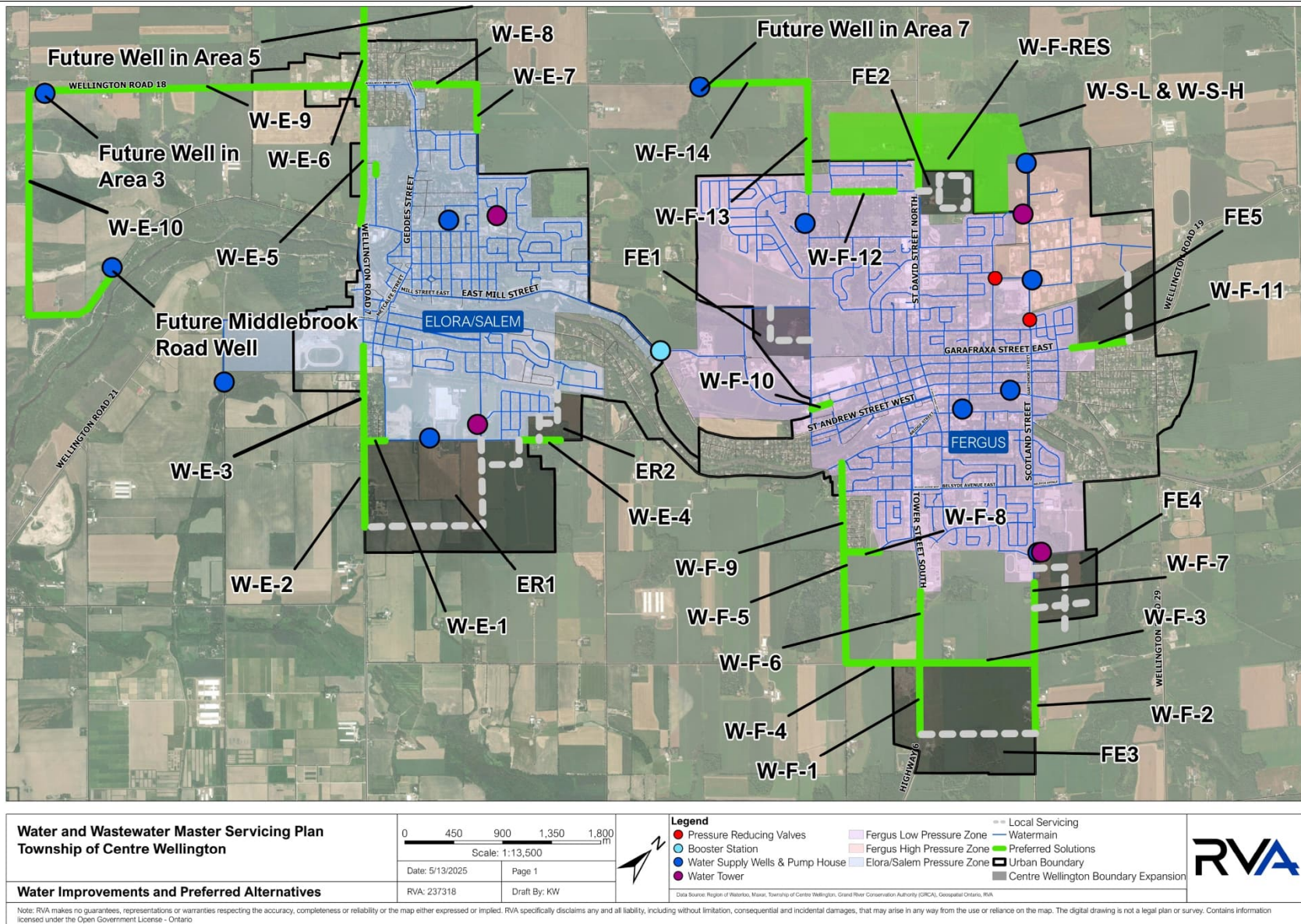
Figure 3-2 Proposed Watermains for Servicing to 2051
