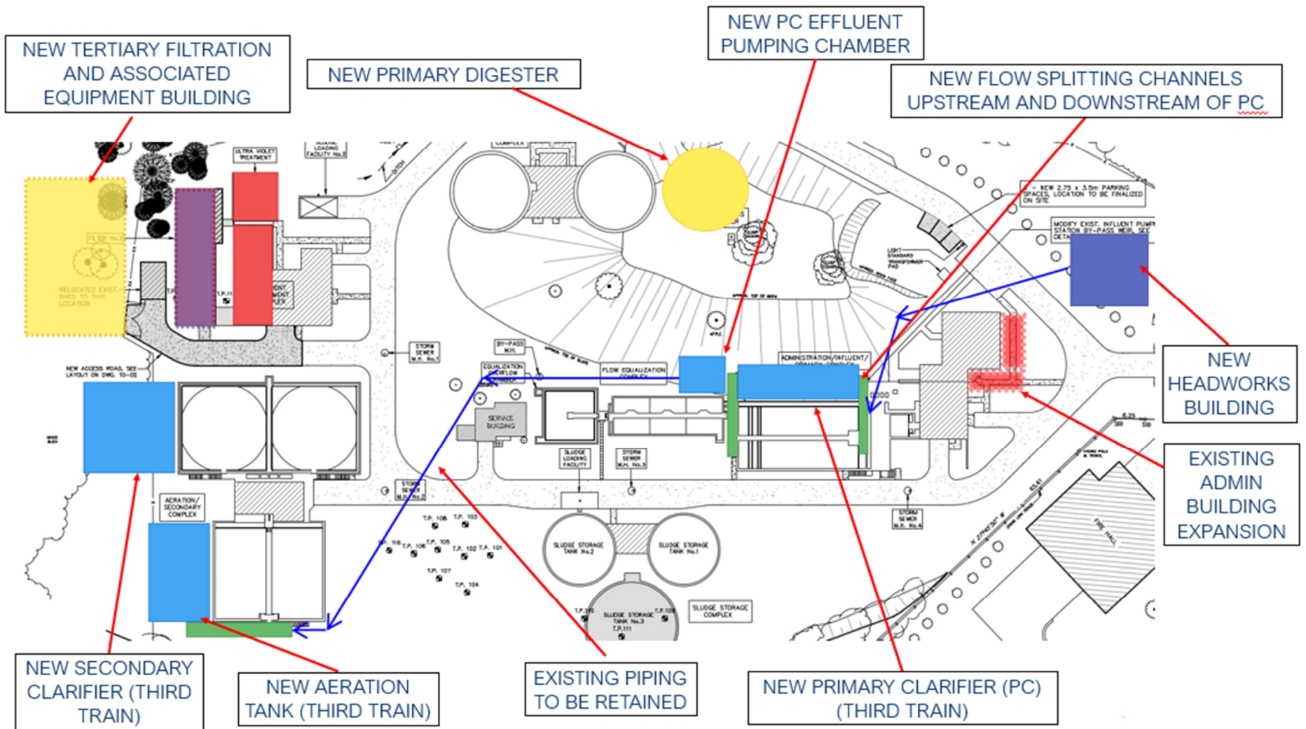
Figure 7-9 Conventional Activated Sludge (CAS) Facility Expansion Layout
