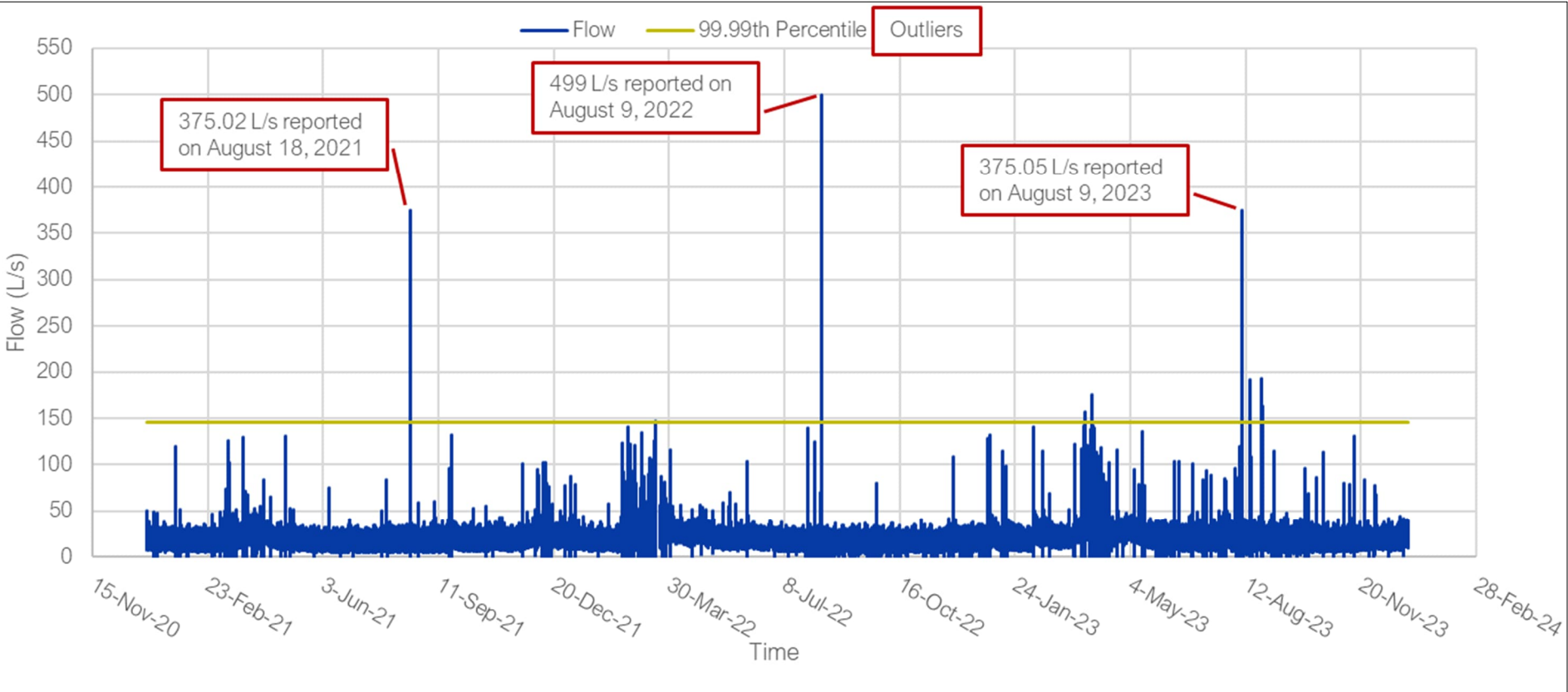
Figure 2-1 Elora WWTP Historical Flow Trend
