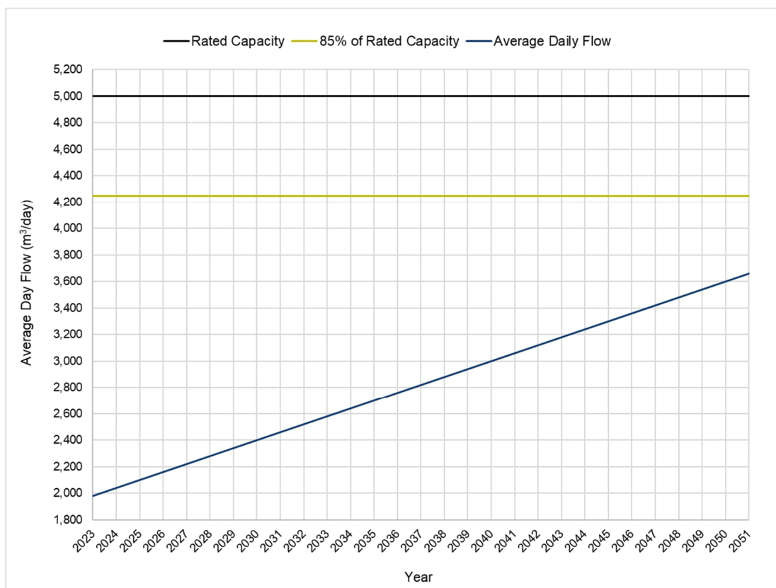
Figure 2-3 Elora WWTS Projected Wastewater Flows
