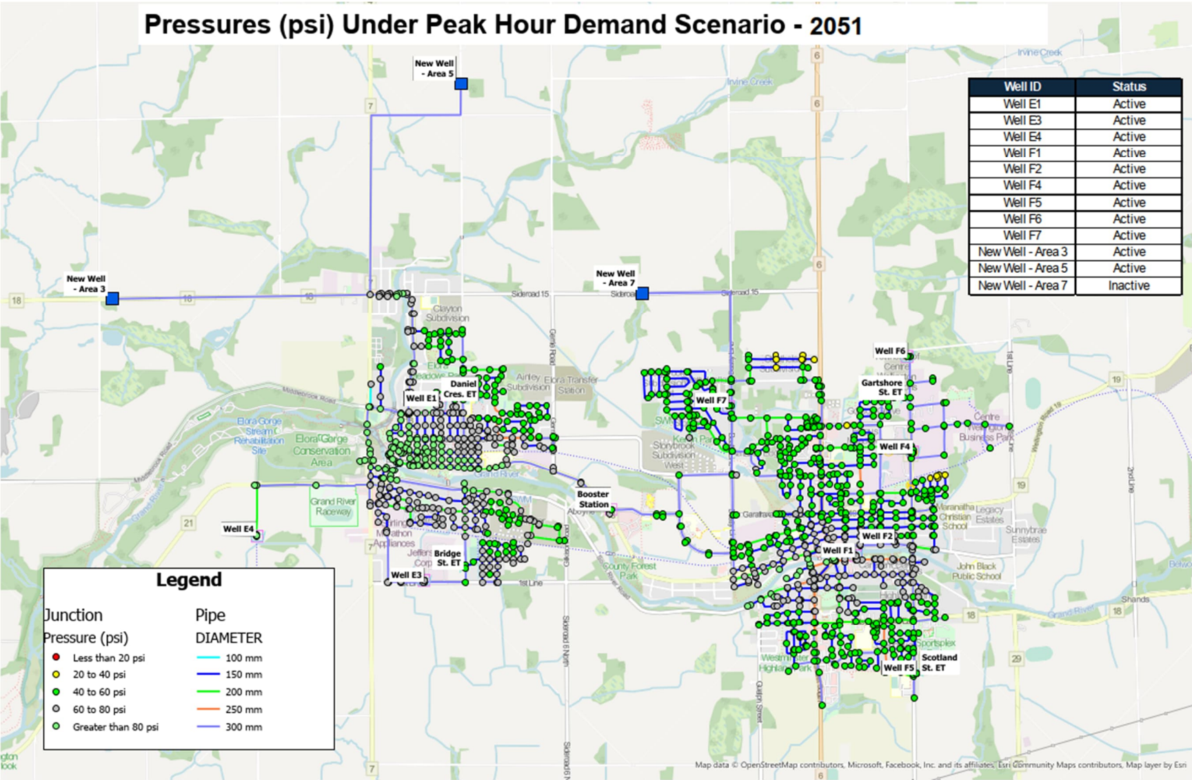
Figure 6-6 Hydraulic Modelling Pressures Under Peak Hour Demand for 2051
