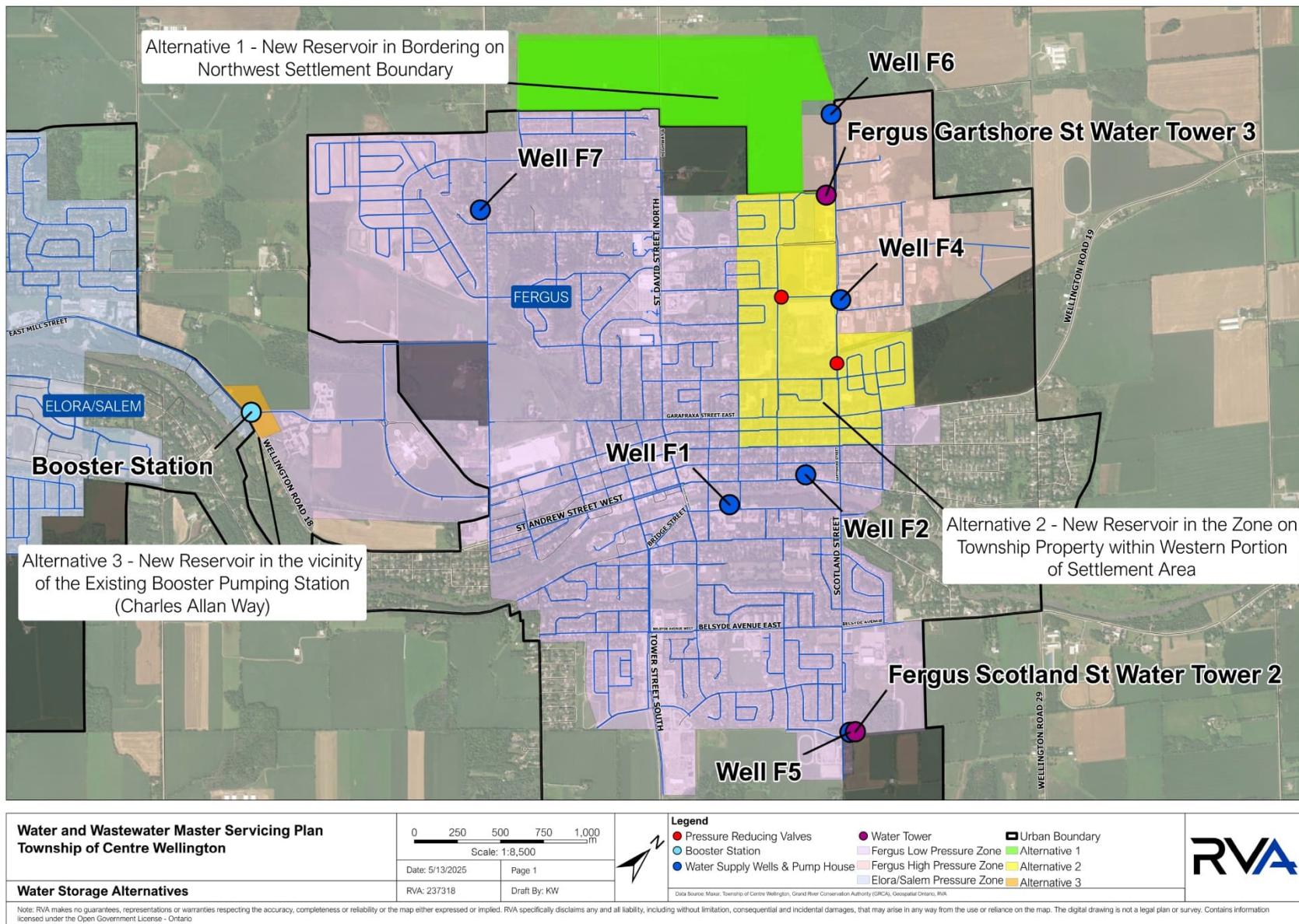
Figure 6-7 Water Storage Options
