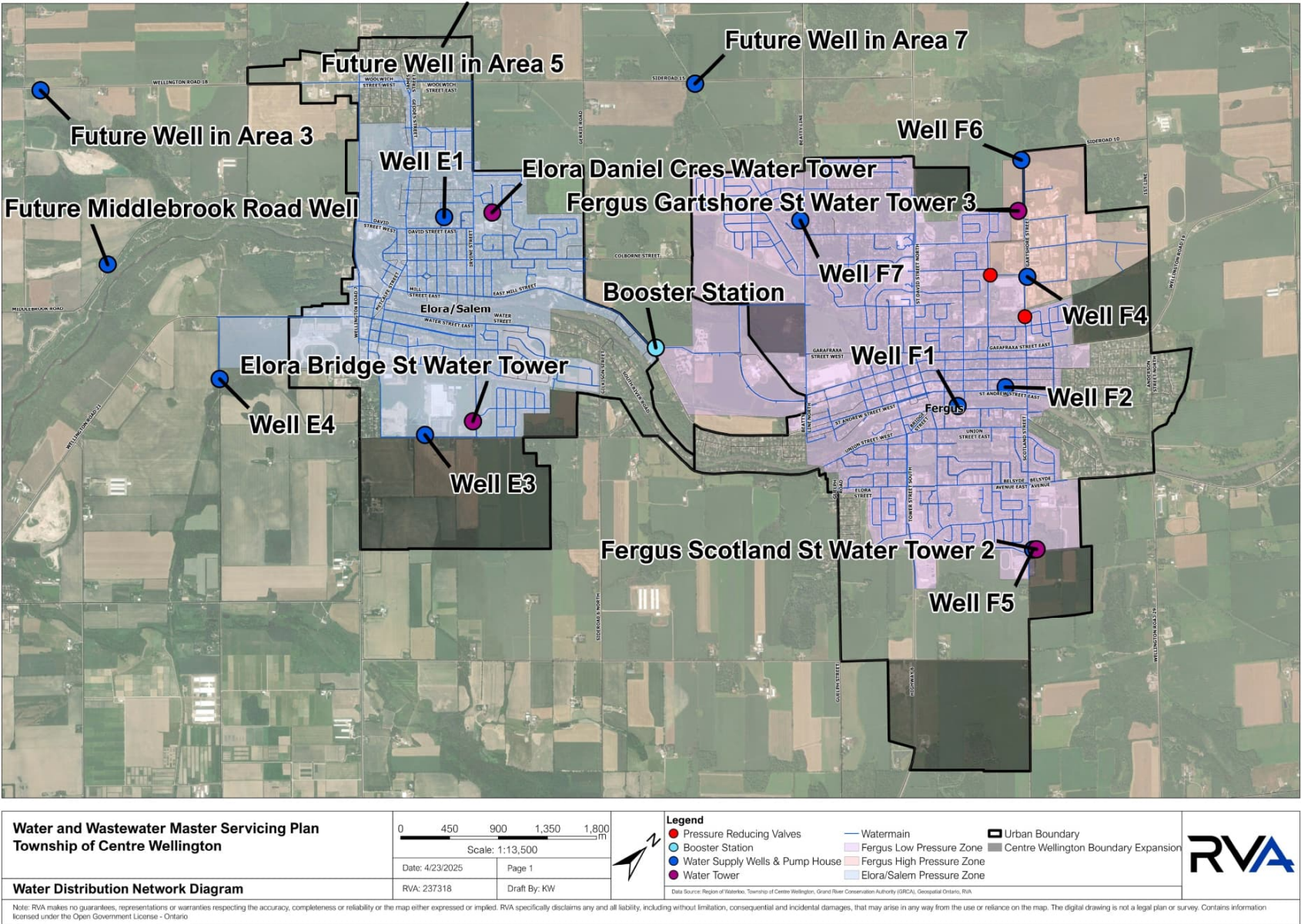
Figure 2-1 Current Water System
