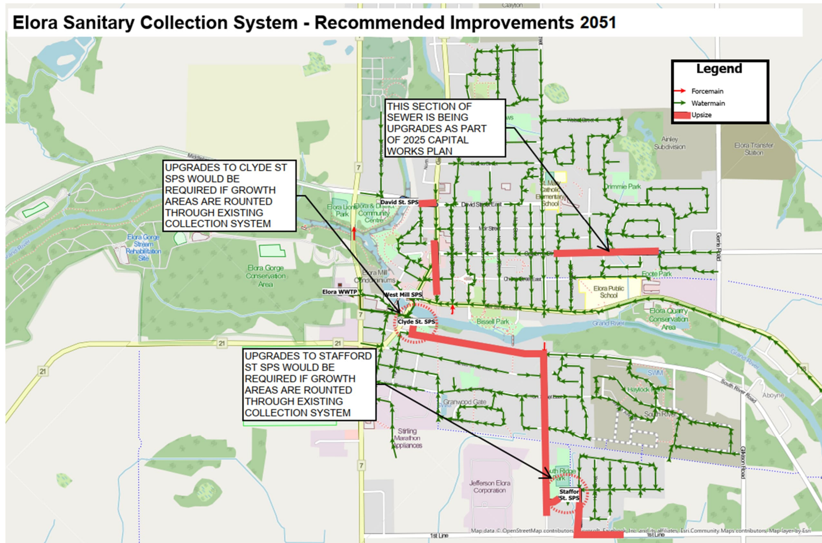
Figure 7-3 2051 Growth Impact on Existing Elora-Salem Collection System
