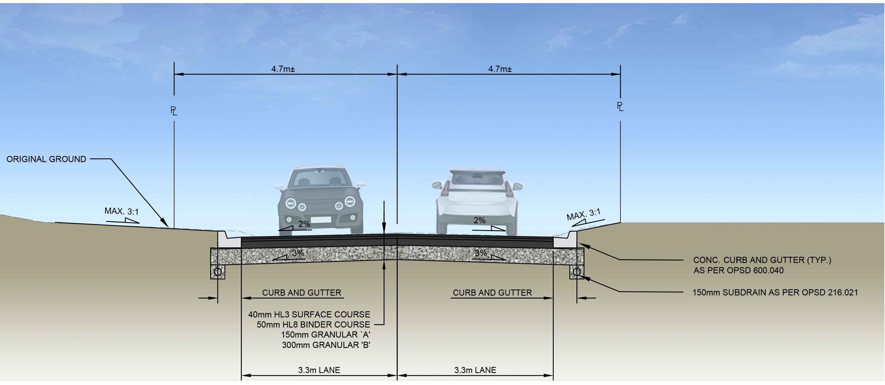
ANNE STREET (SOUTH TO NORTH) TYPICAL SECTION B-B
