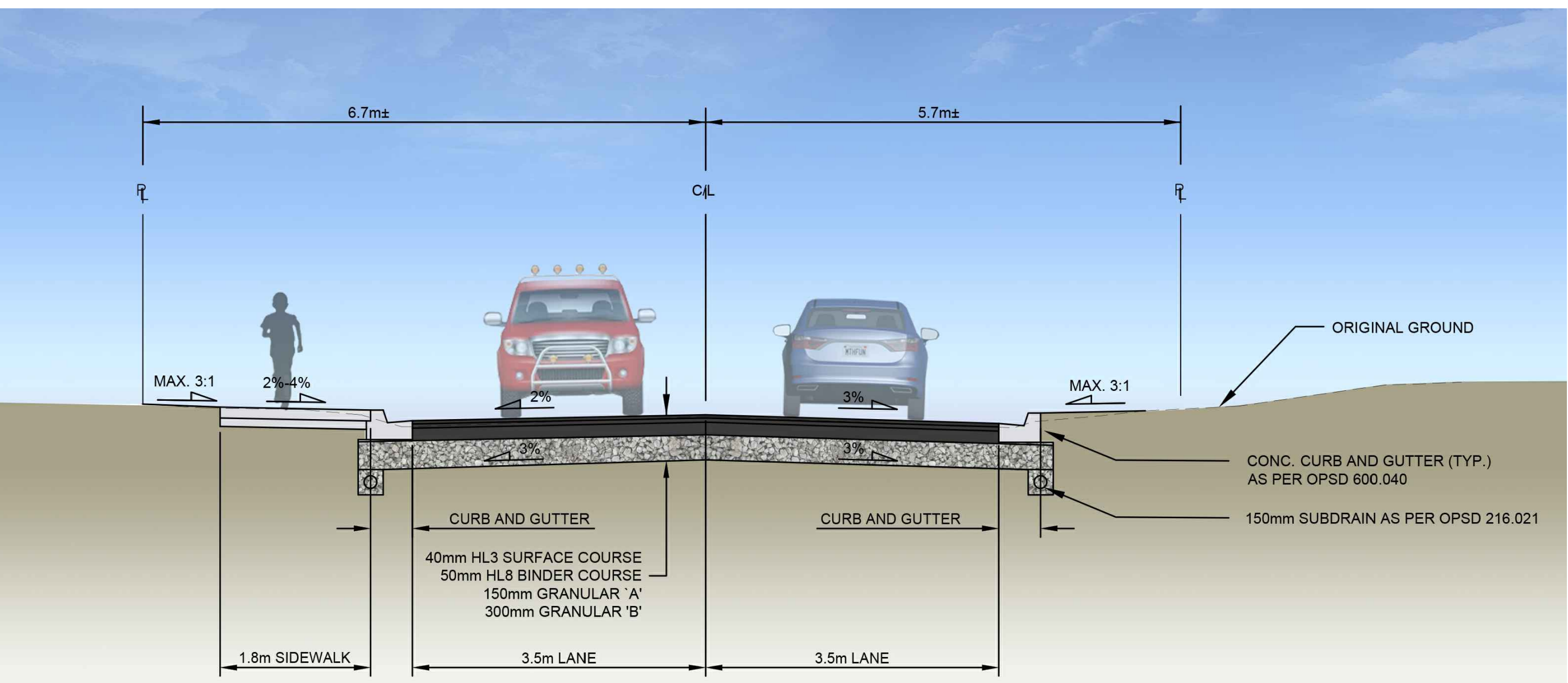
ANNE STREET (WEST TO EAST) TYPICAL SECTION A-A
