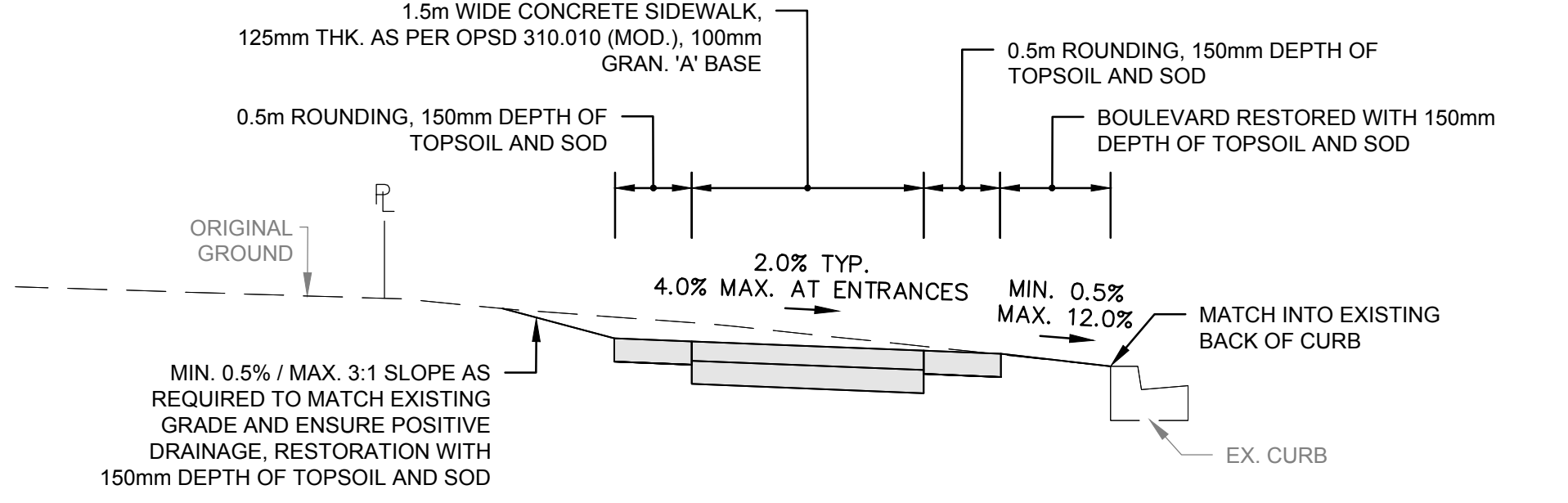
TYPICAL SECTION - UNIVERSITY AVENUE, NORTH SIDE, FROM CAMPBELL STREET TO COTTESMORE AVENUE N.T.S.
