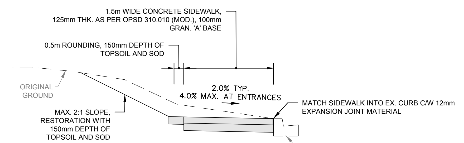
TYPICAL SECTION - HEATH STREET, SIDEWALK ADJACENT TO CURB N.T.S.
