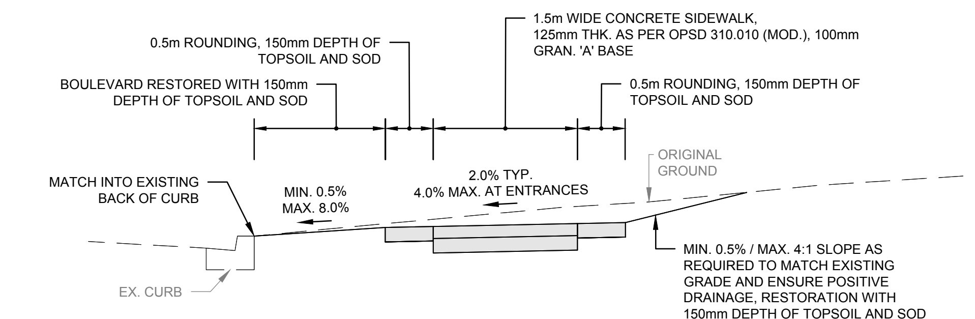
TYPICAL SECTION - MUNROE STREET N.T.S.
