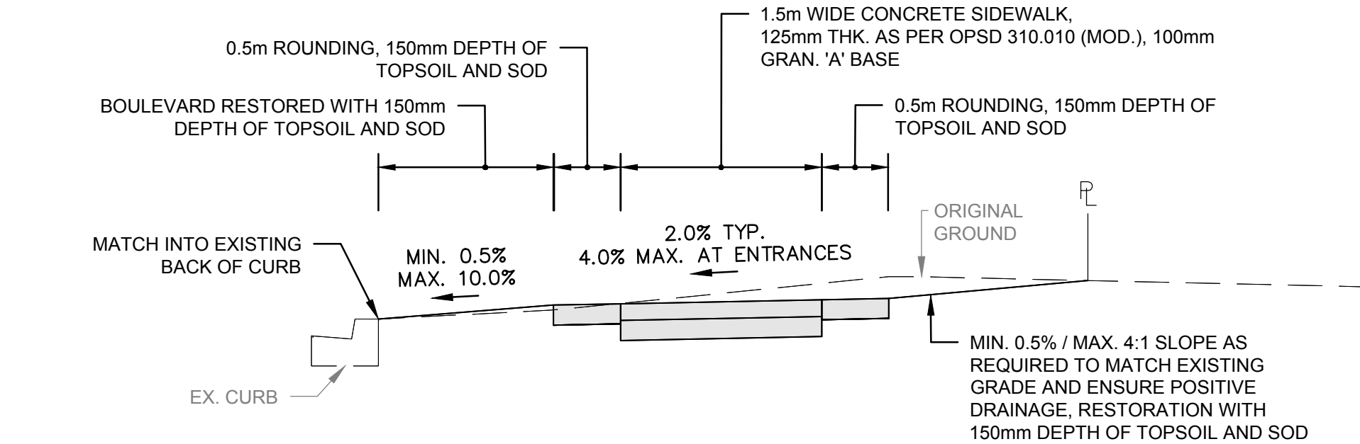
TYPICAL SECTION - UNIVERSITY AVENUE, SOUTH SIDE FROM D'ARCY STREET TO CAMPBELL STREET N.T.S.
