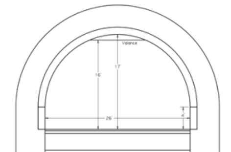
View of Stage Front Proscenium Opening
