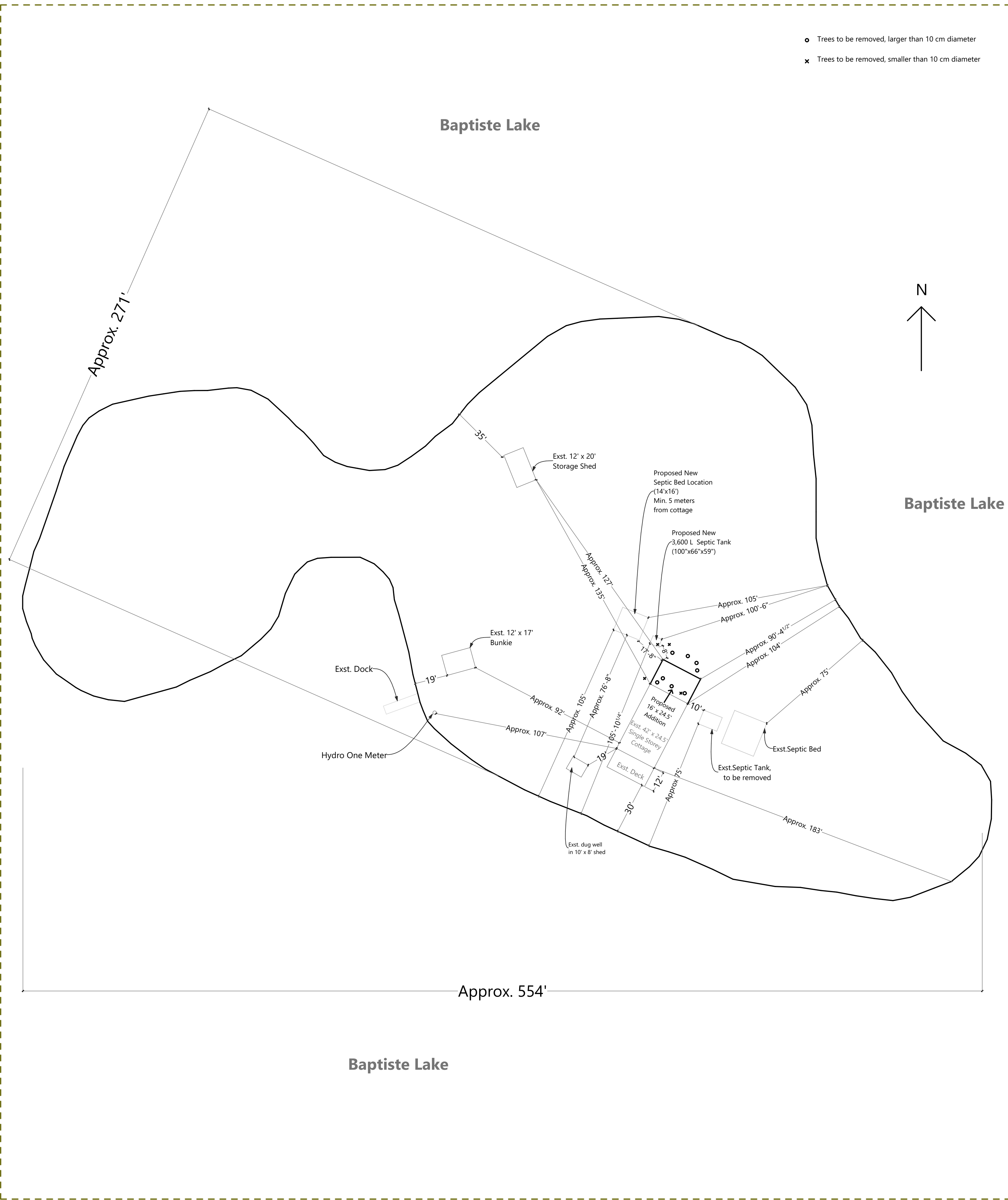
2 Island Site Plan
