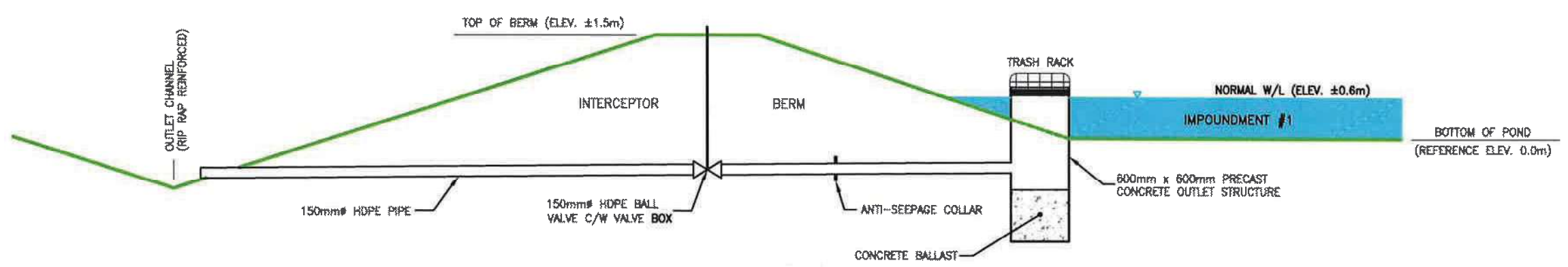
OUTLET SCHEMATIC N T S
