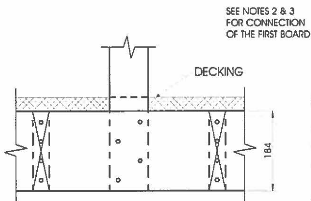
FRONT ELEVATION
