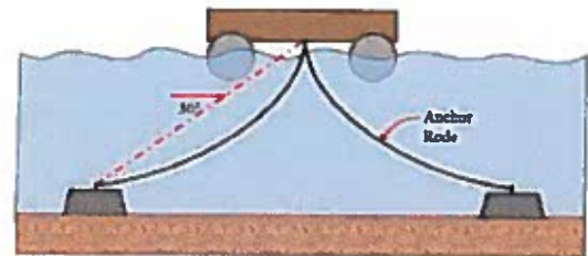
Figure 6.1: Deadman Anchoring Method
